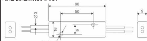
Figure 2: Dimensions of 1x2 or 2x2 Fused Splitter With 3mm Cabled Fibers
